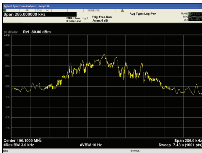
Figure 2-32a. Video filtering
