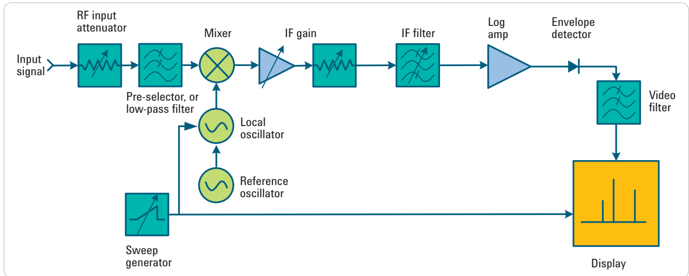
Figure 2-1. Block diagram of a classic superheterodyne spectrum analyzer
