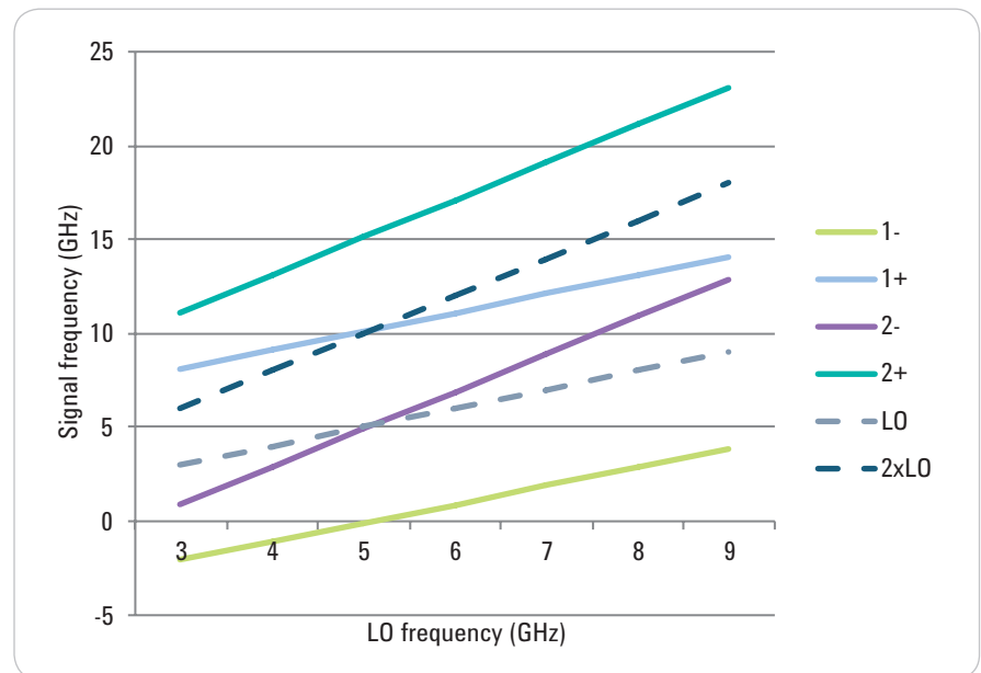
Figure 7-3. Signals in the "1 minus" frequency range produce single, unambiguous responses in the low-band, high-IF case
