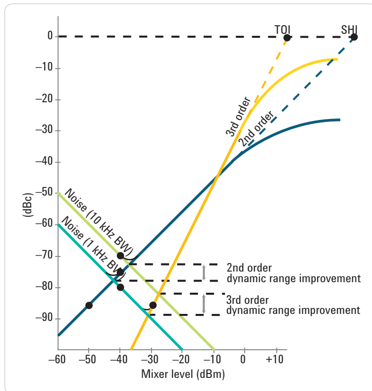
Figure 6-3. Reducing resolution bandwidth improves dynamic range
