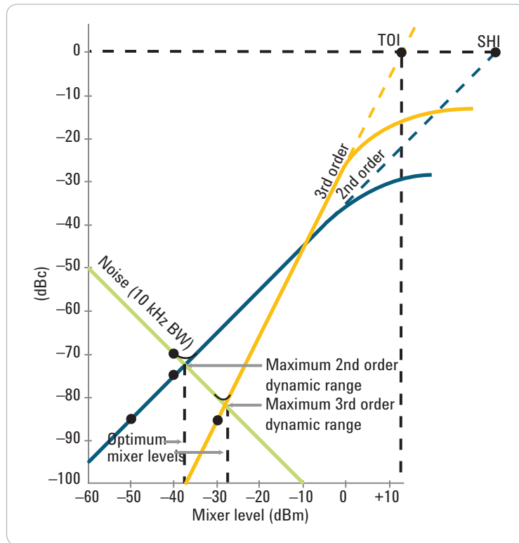
Figure 6-2. Dynamic range versus distortion and noise
