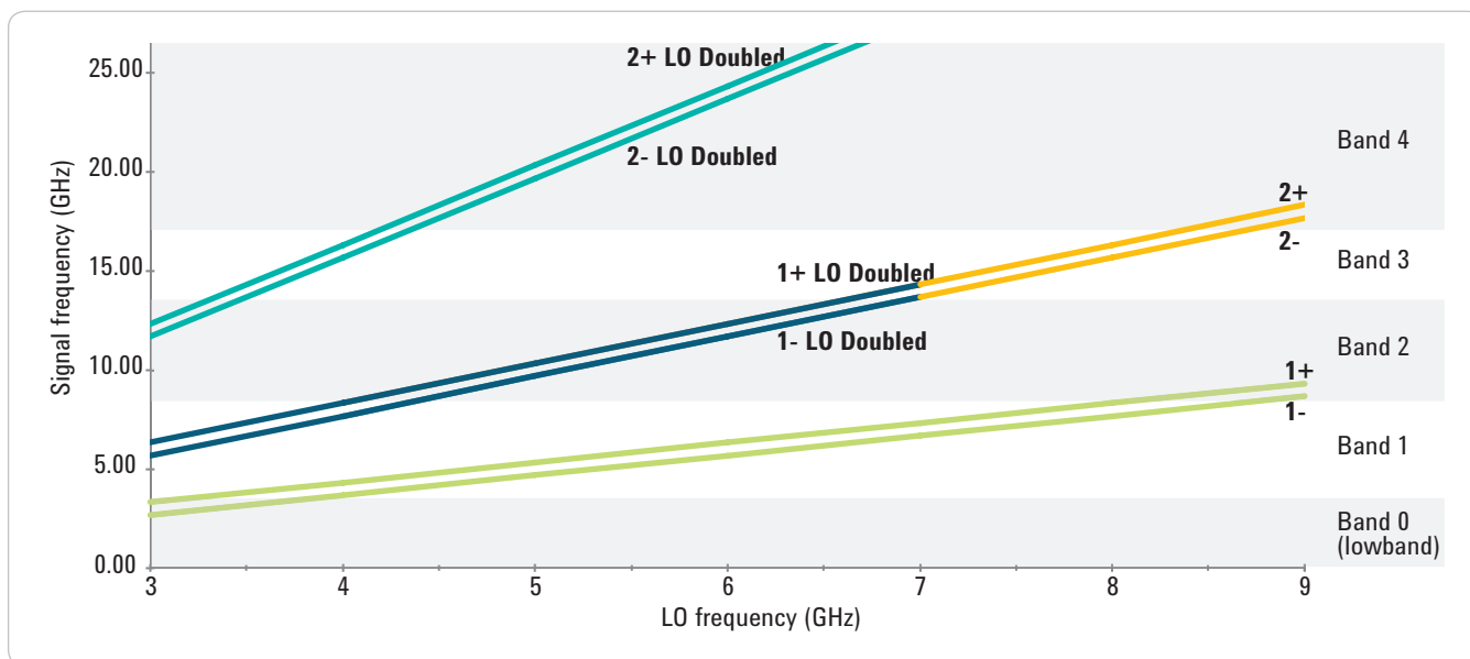
Figure 7-7. X-Series analyzer harmonic bands using LO doubling
