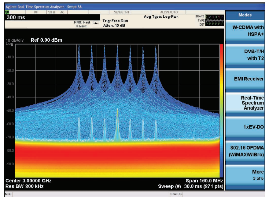
Figure 8-8. Real-time capture of S-band acquisition radar signal
