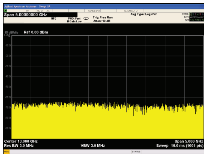
Figure 2-23a. Normal mode
