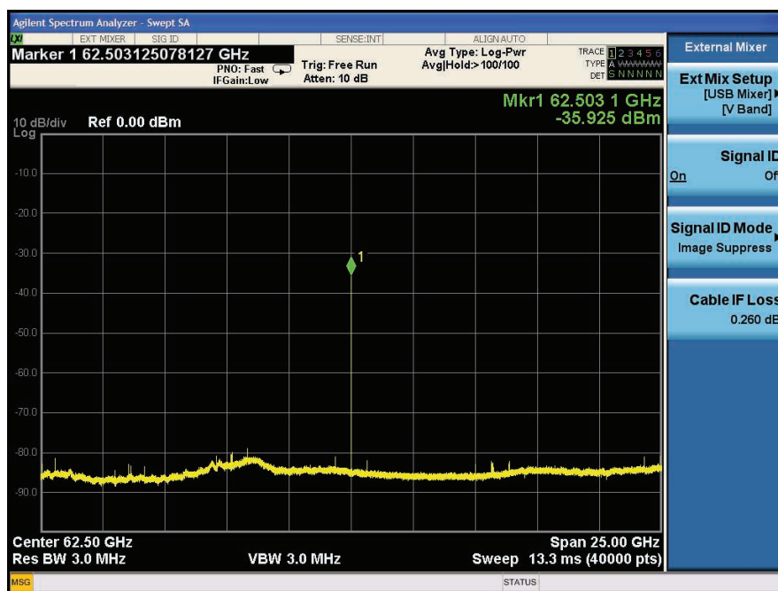
Figure 7-18. The image suppress function displays only real signals
