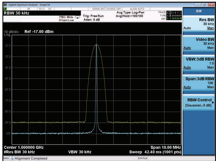
Figure 5-2. Displayed noise level changes as 10 \log (BW_2/BW_1)
