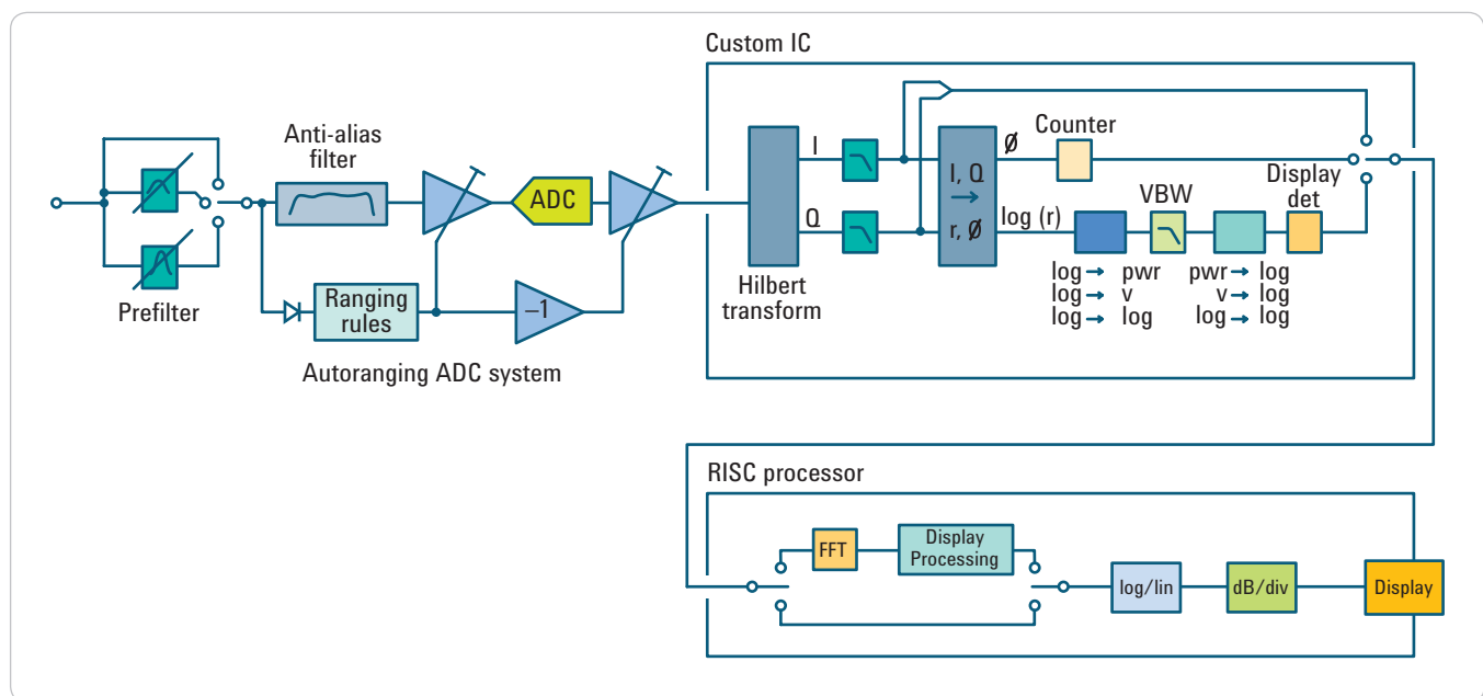
Figure 3-2. Block diagram of the all-digital IF in the Agilent X-Series signal analyzers
