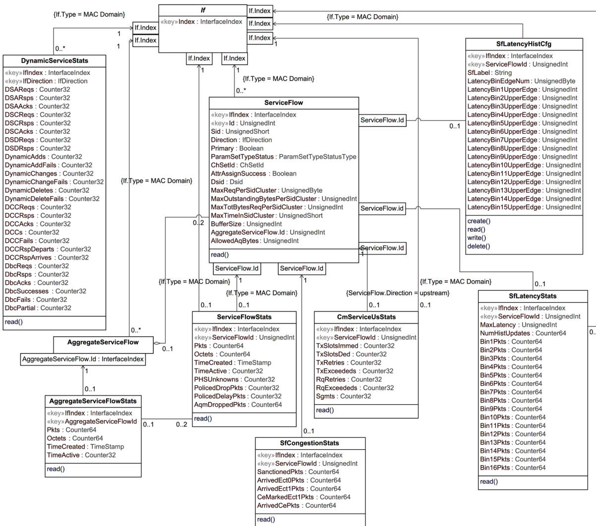
Figure 19 - QoS Statistics Information Model
