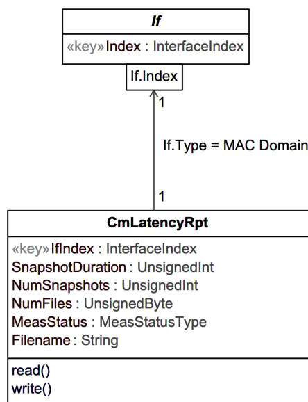
Figure 10 - Latency Report Information Model
