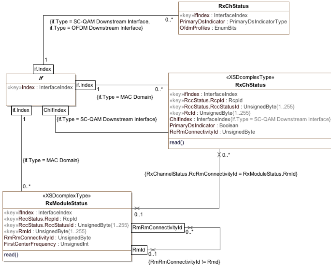
Figure 17 - RCC Status Information Model
