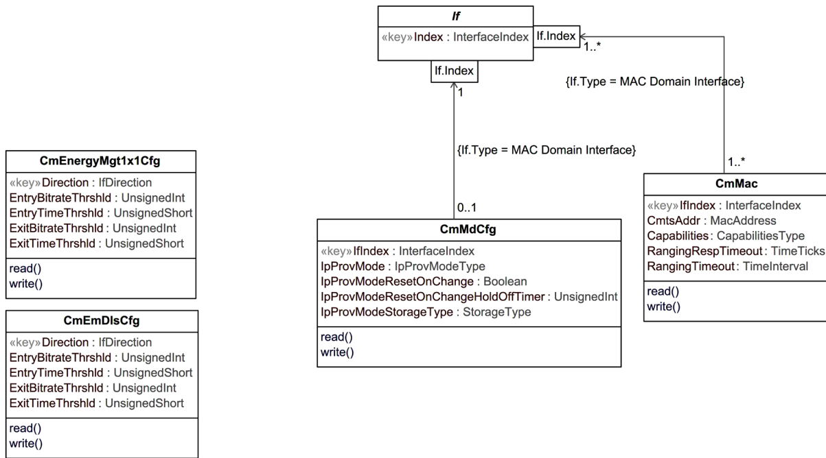
Figure 21 - CM Configuration Information Model
