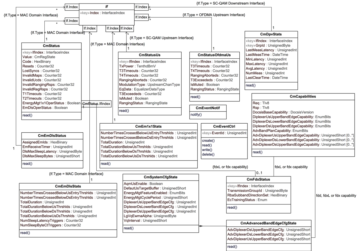
Figure 14 - CM Configuration State and Operational Status Information Model
