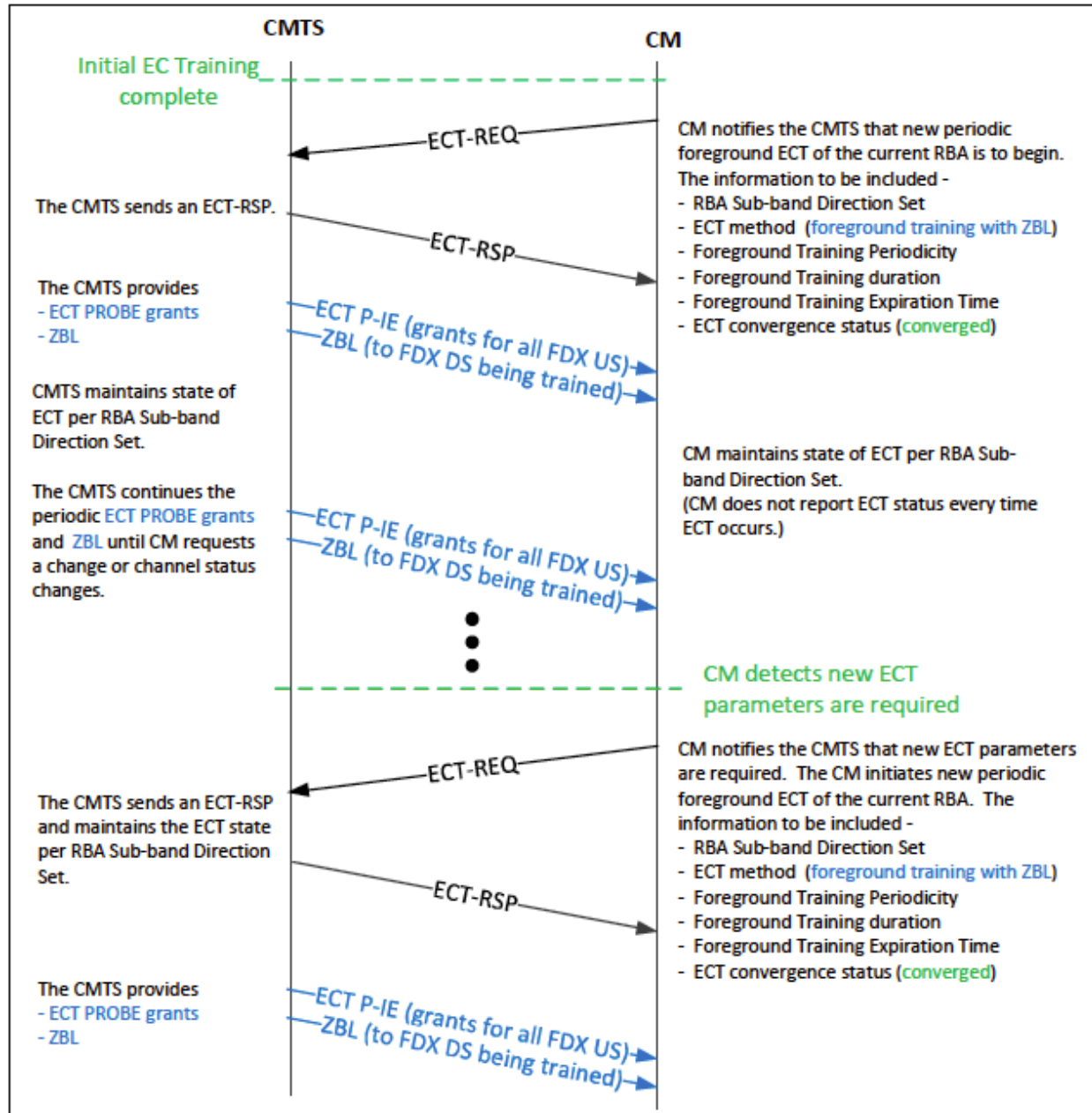
Figure 276 - Periodic Foreground Training with ZBL
