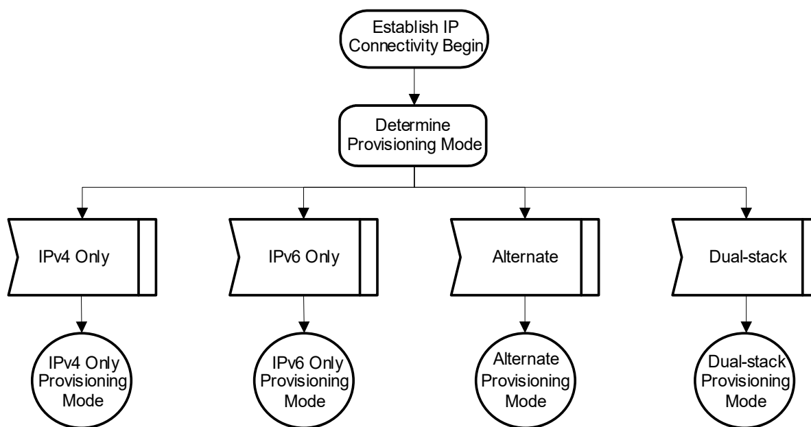
Figure 157 - Establish IP Connectivity
