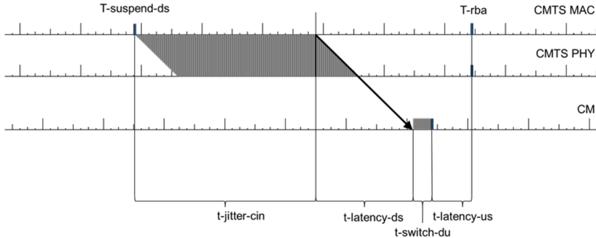
Figure 280 - T\text{-suspend-ds} RPHY Timing
