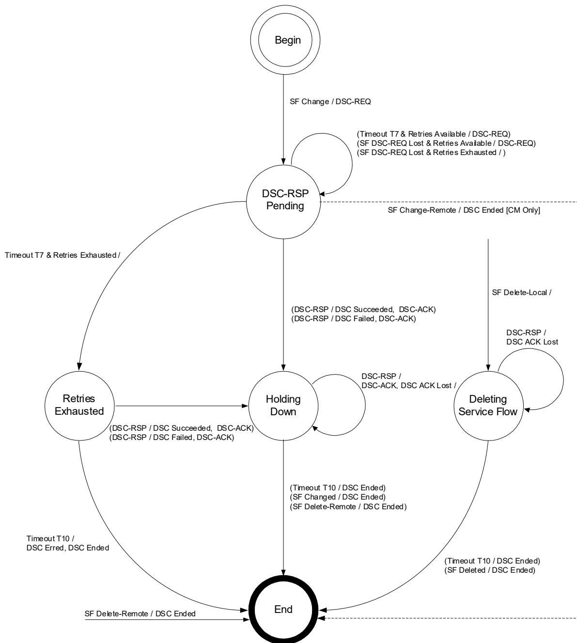
Figure 203 - DSC-Locally Initiated Transaction State Transition Diagram
