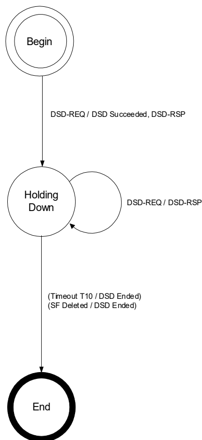
Figure 206 - Dynamic Deletion (DSD)-- Remotely Initiated Transaction State Transition Diagram
