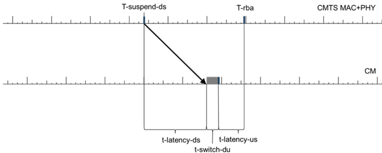
Figure 281 - T\text{-suspend-ds} CMTS timing
