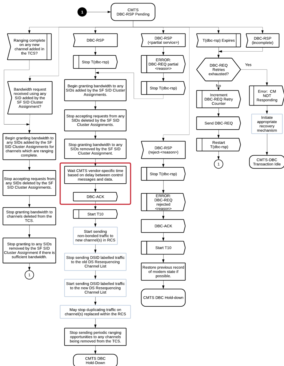
Figure 244 - CMTS DBC-RSP Pending
