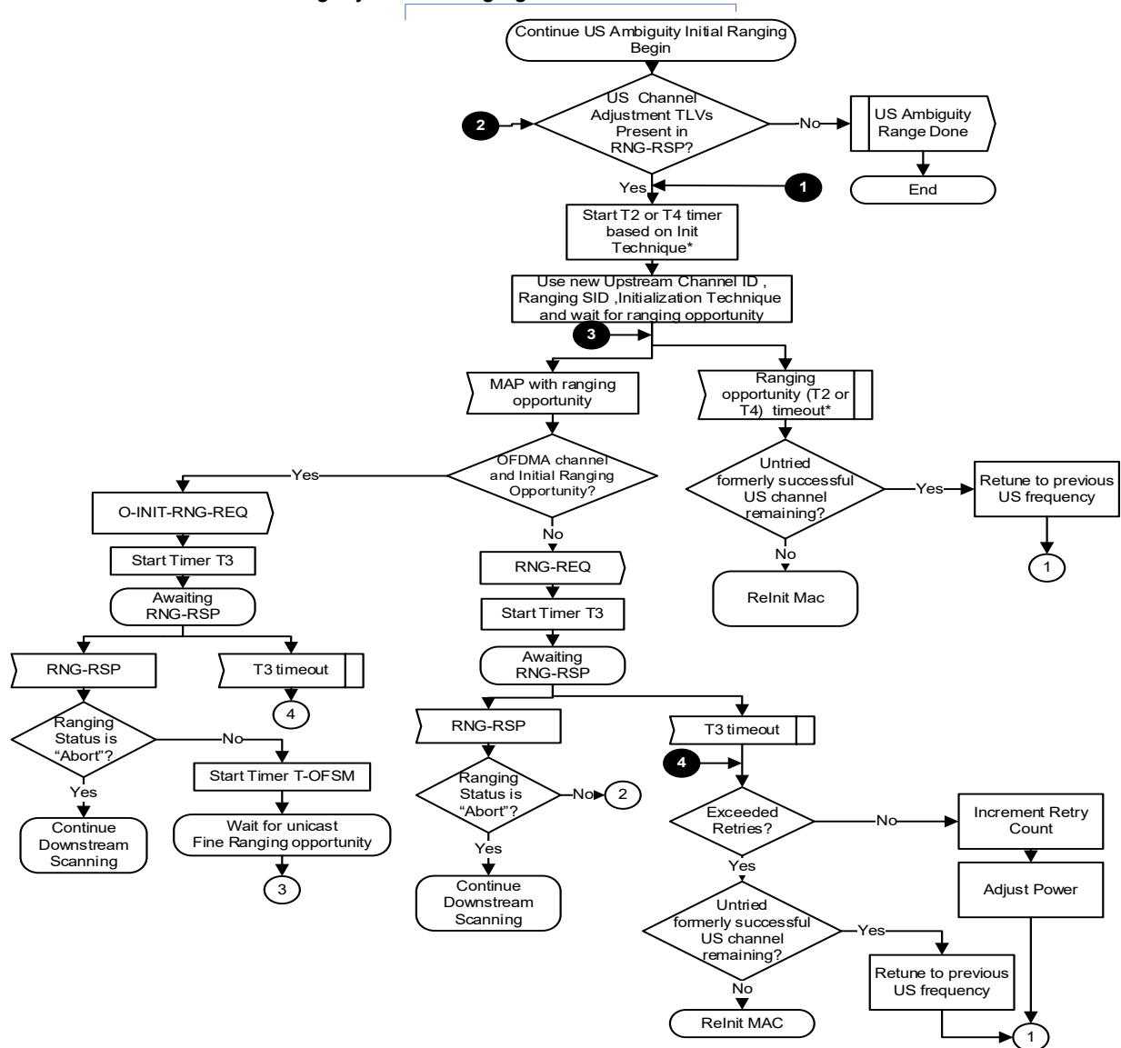
Figure 151 - Continue US Ambiguity Initial Ranging
