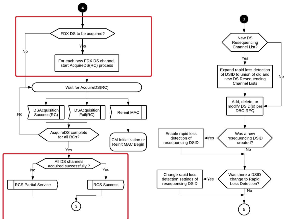
Figure 247 - CM DBC-RSP (part 1b)
