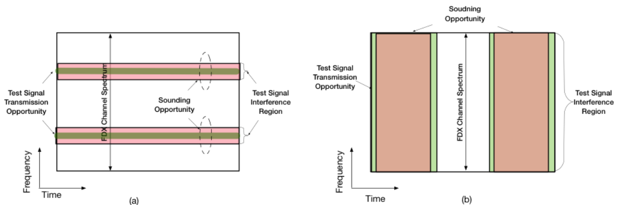
Figure 265 - Sounding Opportunities (a) CWT Sounding (b) OUDP Sounding
