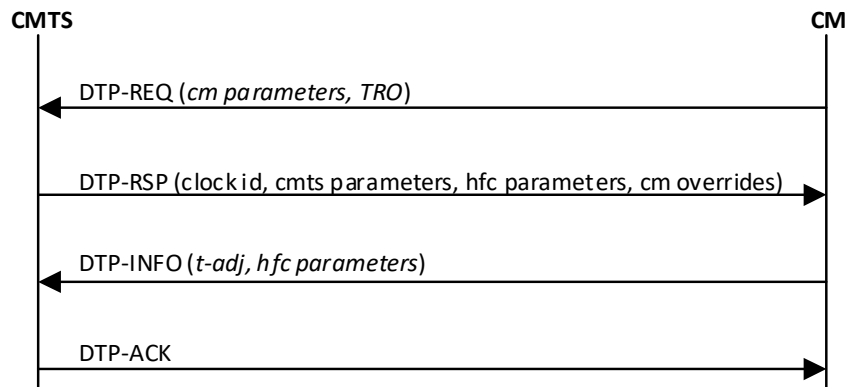
Figure 197 - CM is DTP Master
