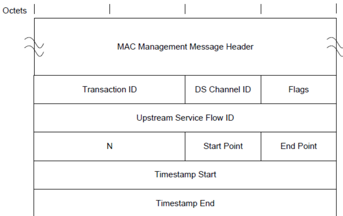
Figure 73 - DPV-REQ MAC Message
