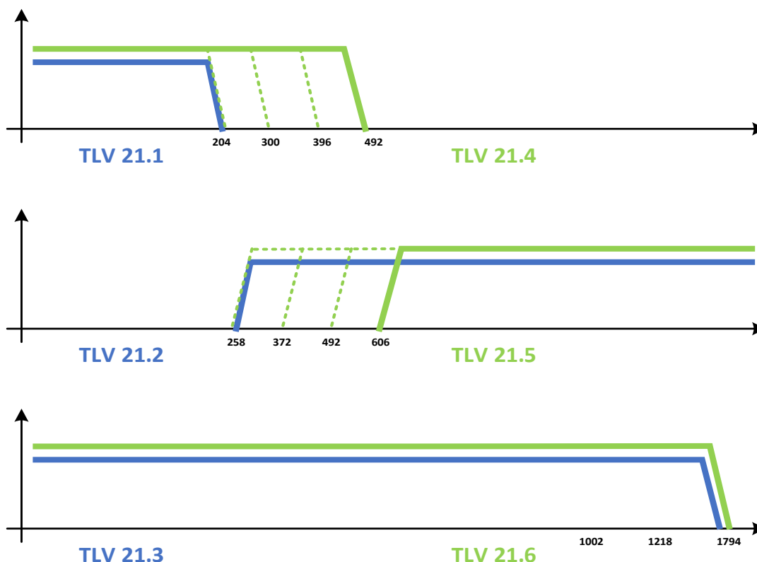
Figure 69 - Band Edge sub-TLVs Behavior
