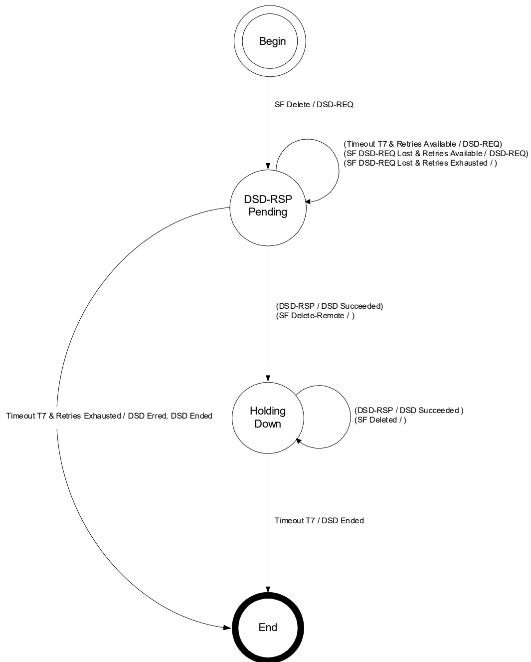
Figure 205 - DSD-Locally Initiated Transaction State Transition Diagram
