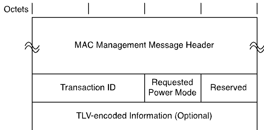
Figure 78 - Energy Management Request Message
