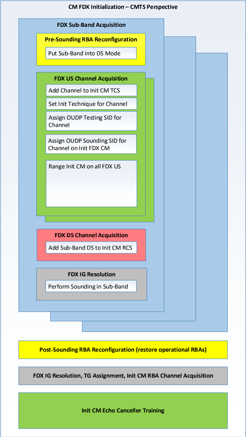
Figure 262 - CM FDX Initialization Framework
