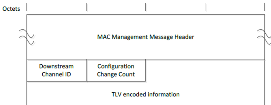
Figure 81 - OFDM Channel Descriptor
