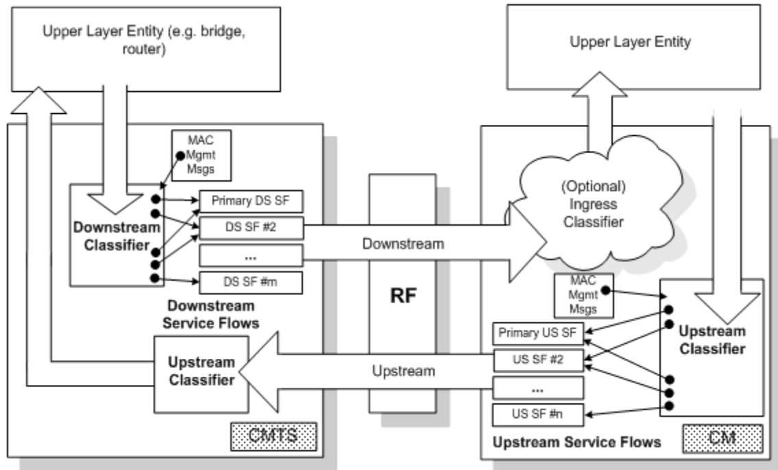
Figure 116 - Classification within the MAC Layer
