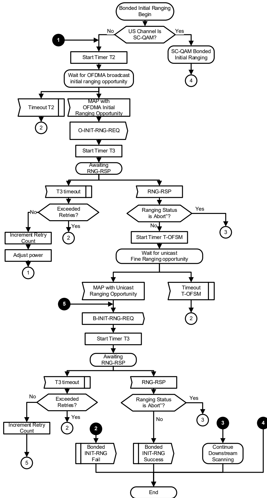
Figure 149 - Bonded Initial Ranging
