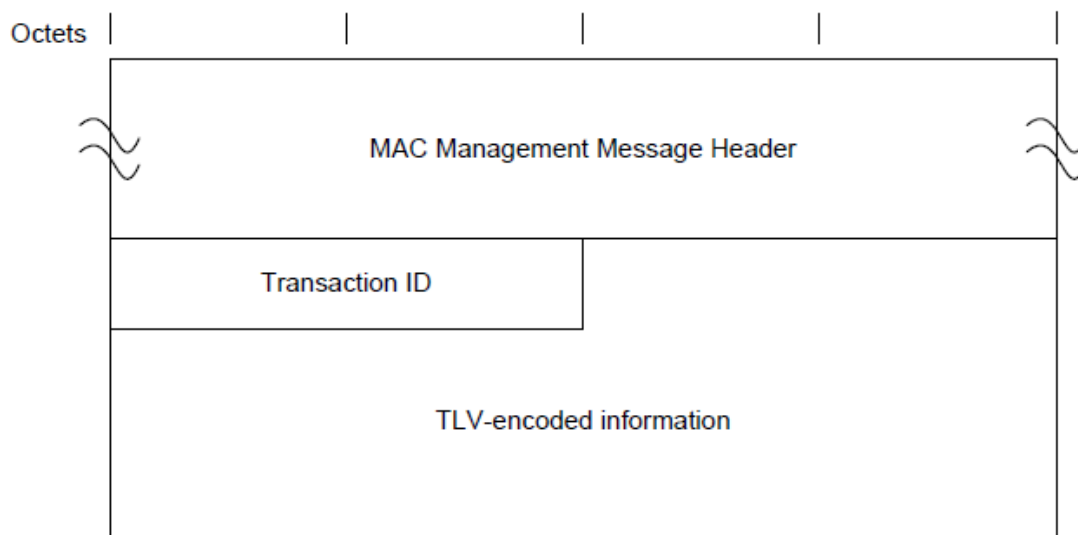
Figure 72 - Dynamic Bonding Change Acknowledge Message
