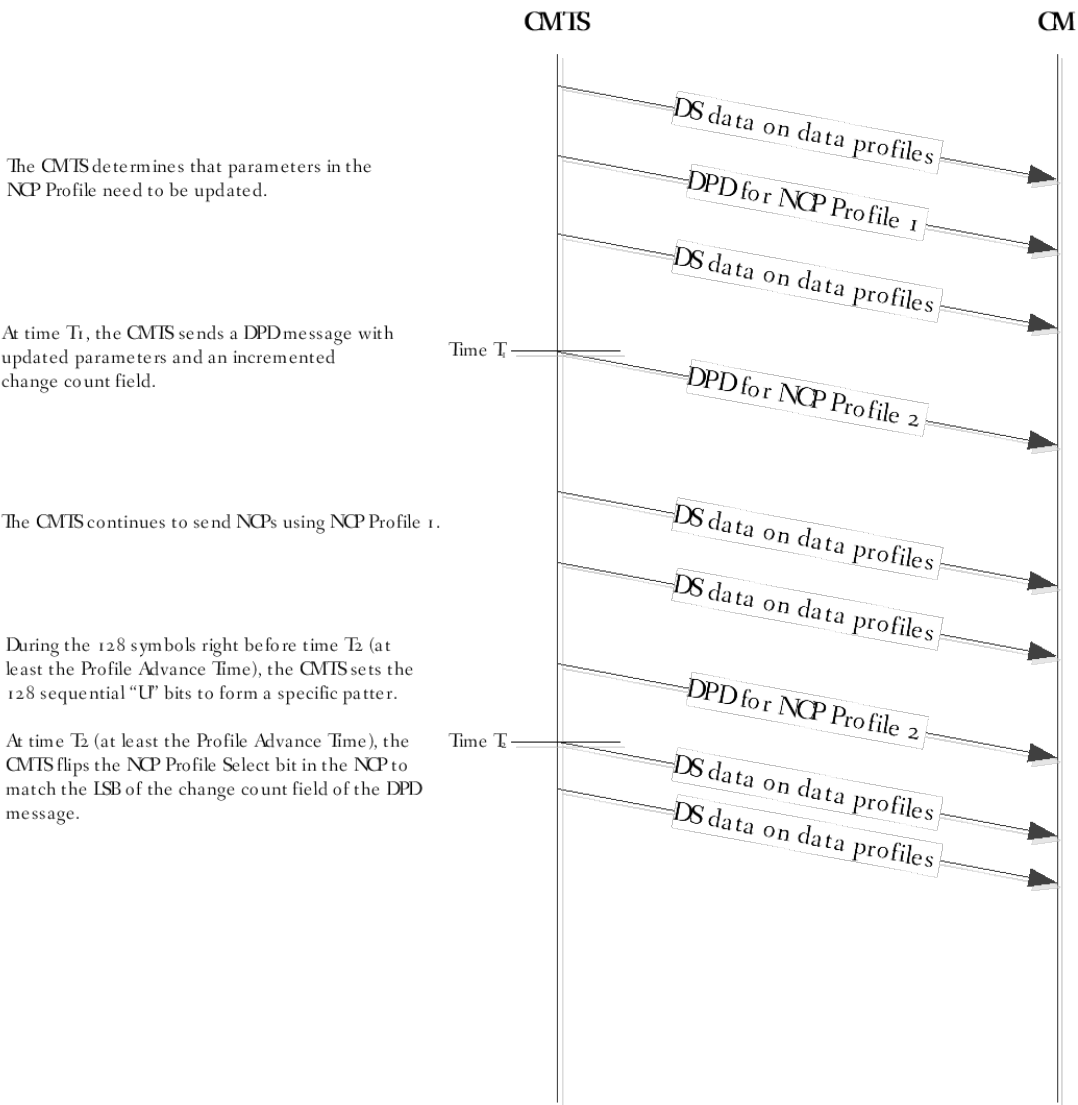
Figure 321 - DPD Change to the NCP Profile
