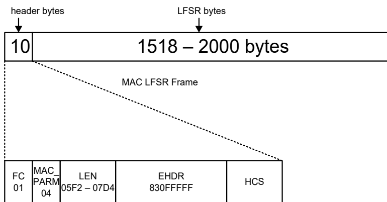
Figure 184 - MAC LFSR Frame
