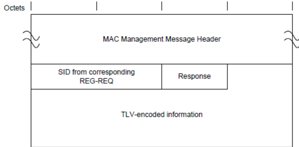
Figure 54 - Registration Response Format
