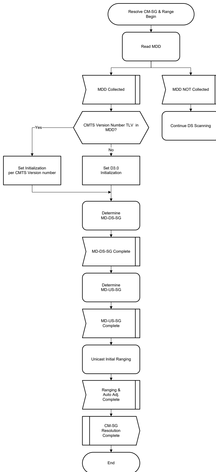
Figure 144 - Resolve Service Group (SG) and Range
