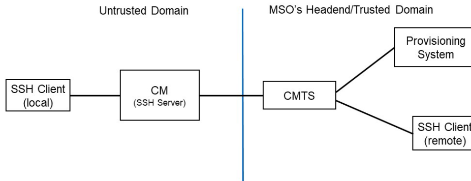
Figure 20 - SNMP-Based Authentication Architecture
