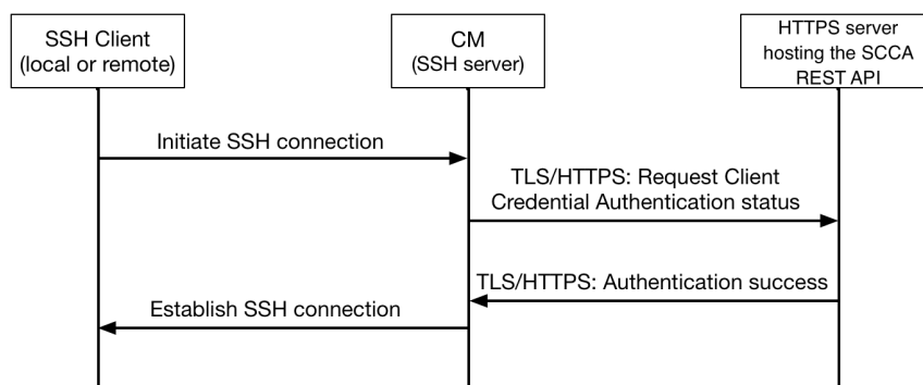
Figure 19 - TLS-based Message Flow
