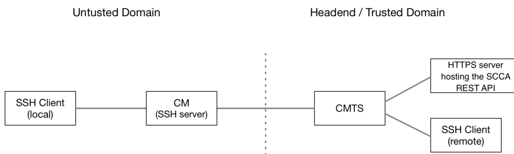
Figure 18 - TLS-based Authentication Architecture
