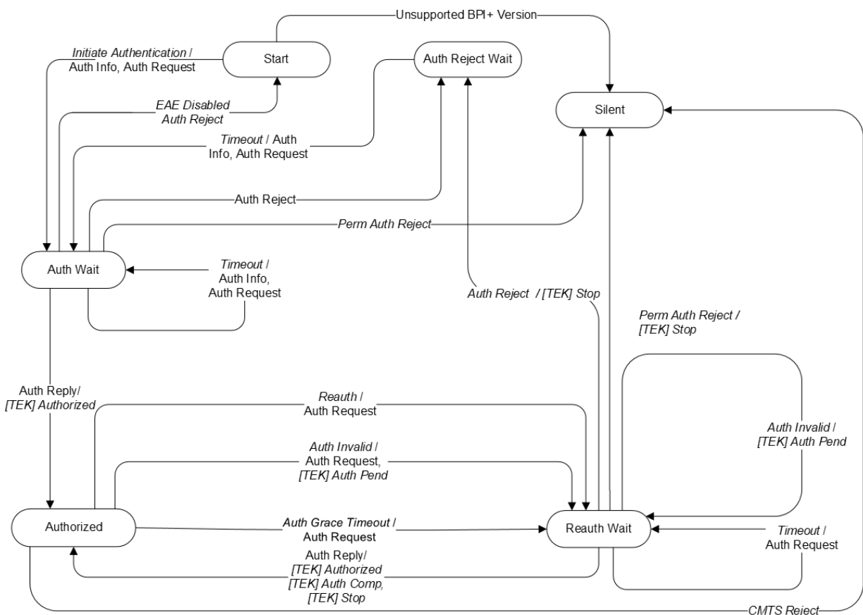
Figure 8 - Authorization State Machine Flow Diagram
