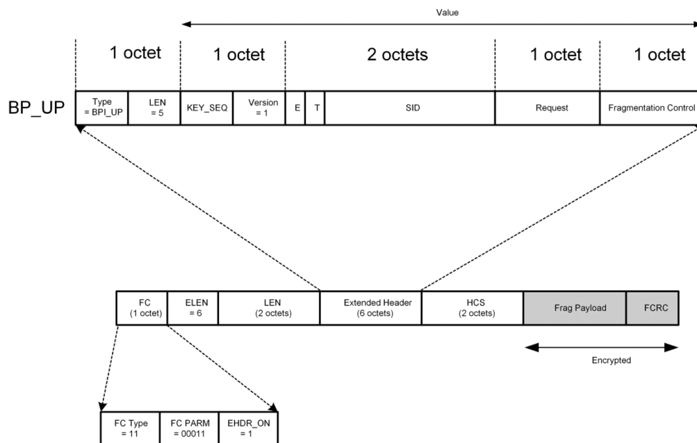
Figure 5 - Format of a DOCSIS MAC Fragmentation Frame with an Encrypted Payload
