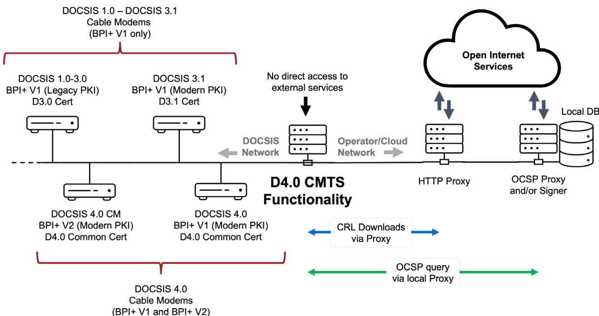
Figure 23 - Example Deployment with Revocation Checking Support and Local Overrides
