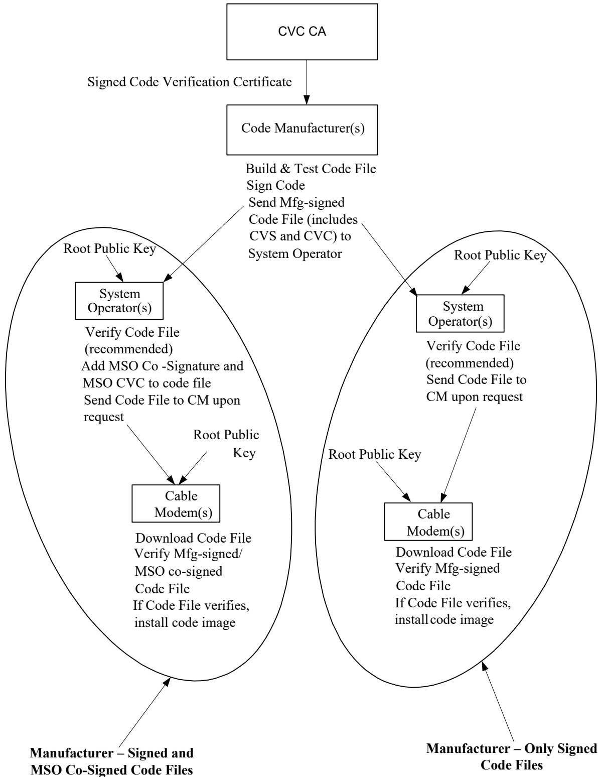
Figure 15 - Typical Code Validation Hierarchy
