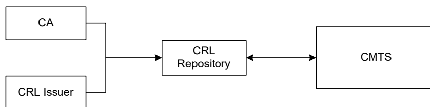
Figure 13 - CRL Framework
